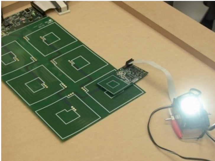
Figure 2: Matrix with multiple transmitting coils for high coverage. Photo © Fraunhofer ENAS
