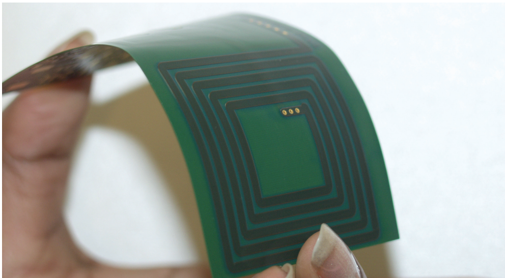
Figure 1: Inductive power receiver on flexible carrier material. Photo © Fraunhofer ENAS
