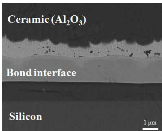
SEM cross section of a Si-ceramic bond interface.
